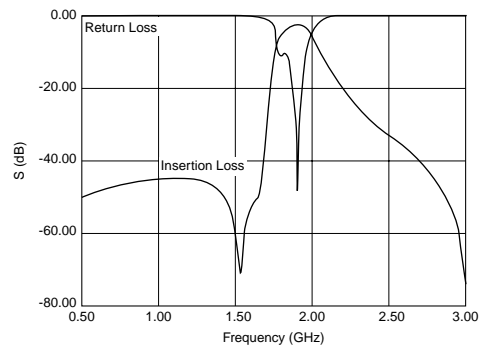
Frequency Characteristics
